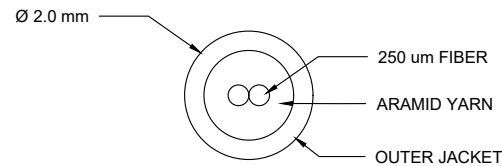
VIEW B CROSS SECTION NOT TO SCALE
