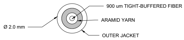
VIEW A CROSS-SECTION NOT TO SCALE
