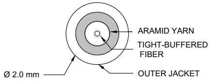
SIMPLEX CABLE CROSS SECTION NOT TO SCALE
